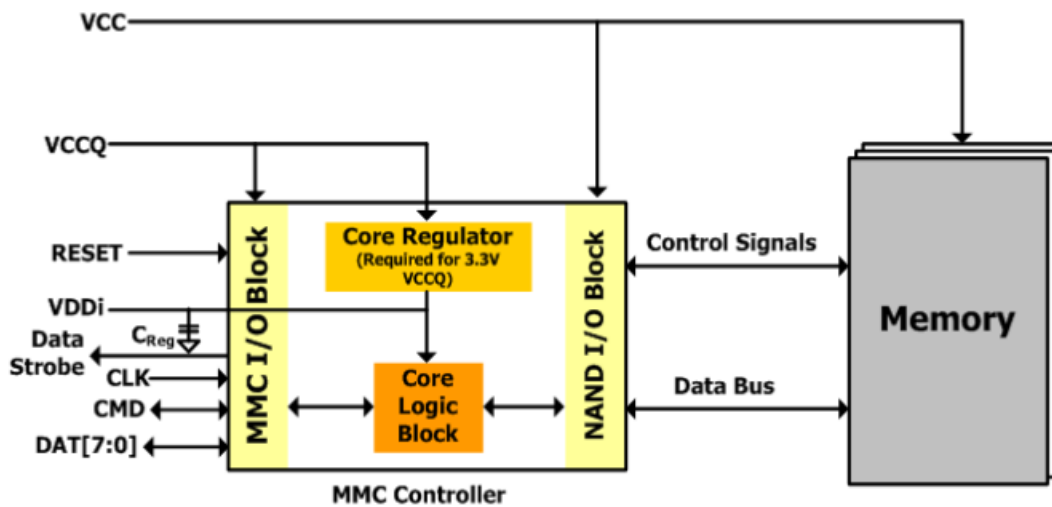
Figure 1 – eMMC Block Diagram
