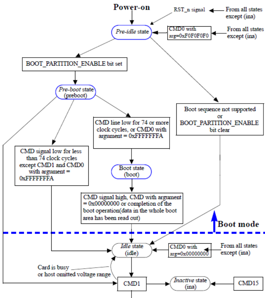
Figure 5 – State diagram (boot mode)*
