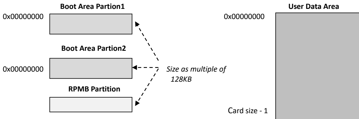
Figure 2 – e-MMC memory organization at time zero
