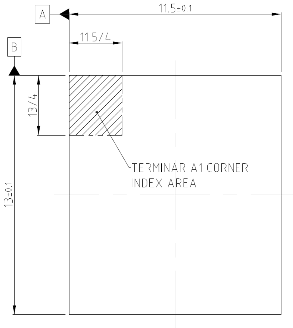
Figure 6 – 11.5 x 13.0 x 1.0mm Top View
