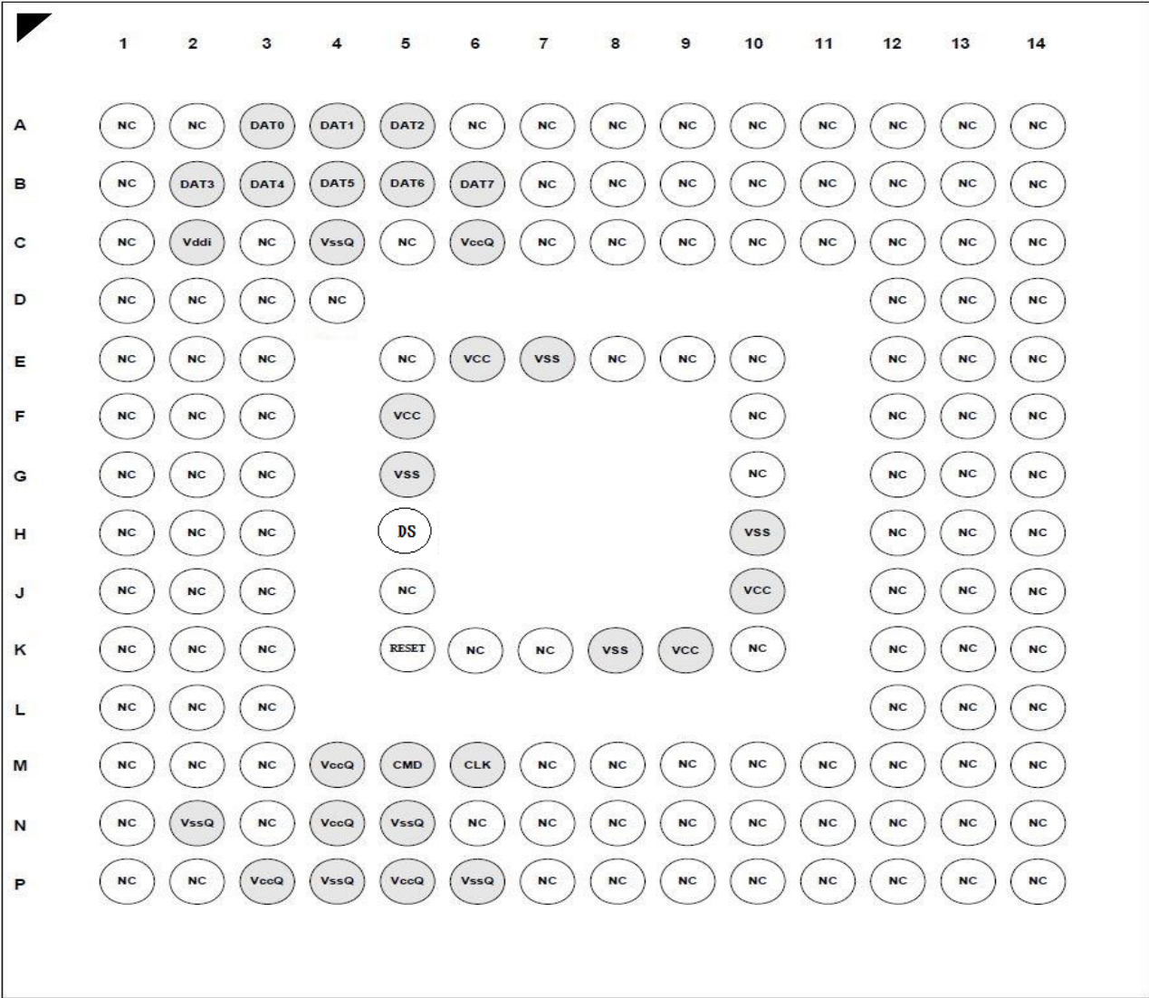
Figure 8 – FBGA153 Package Connection (top view through package)
