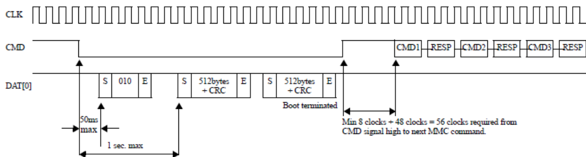
Figure 3 – State diagram (boot mode)
