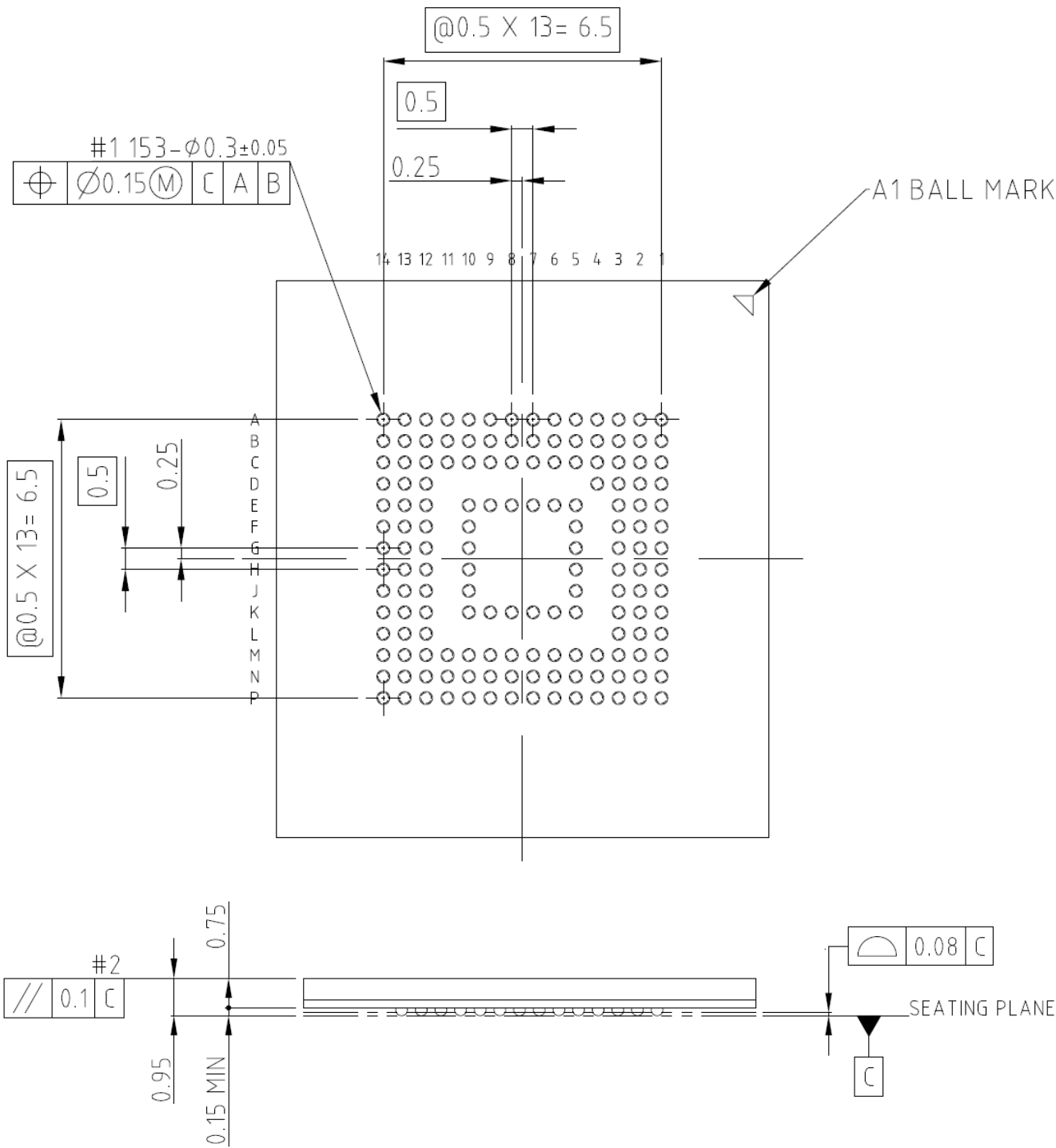
Figure 7 – 11.5 x 13.0 x 1.0mm Bottom & side View
